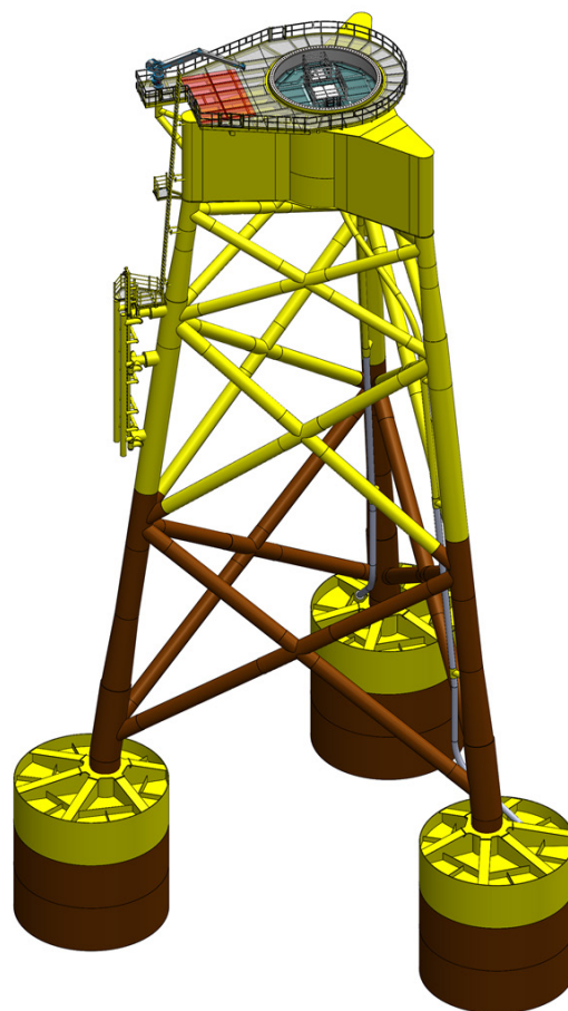
Suction Bucket Jacket
